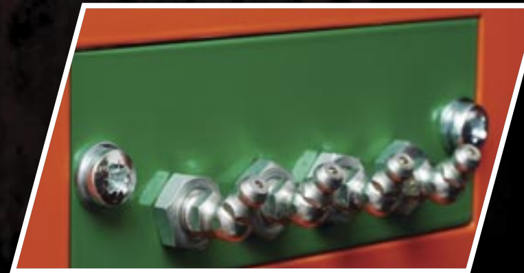
Grease Port Maintenance made easy - convenient central greasing for all bearings.
