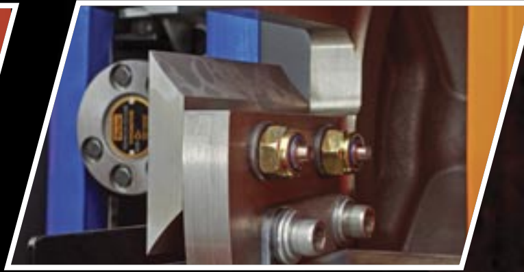
Reversible Blades Unique double half-cut chipping system with double sided, hollow ground blades - exceptional cutting performance, processing.
